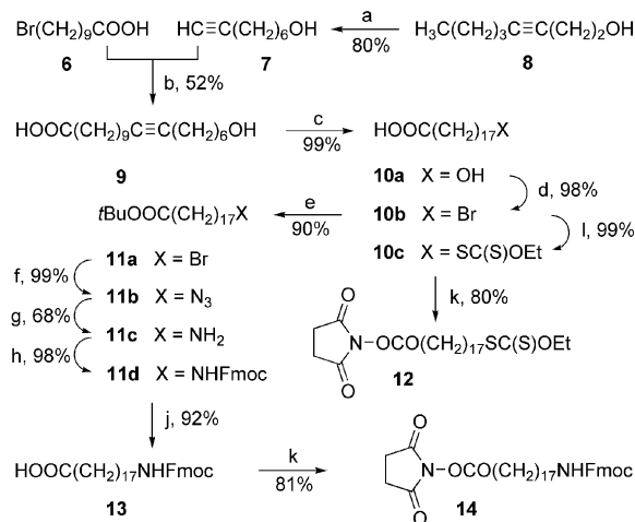
Scheme 4. Active esters 12 and 14 of N -protected \omega -amino- and S -protected \omega -mercaptostearic acids: a) \text{KH} , \text{NH}_2(\text{CH}_2)_2\text{NH}_2 , 80 °C, 5 h; b) \text{LiNH}_2/\text{liq. NH}_3 , -33 °C, 18 h; c) \text{H}_2 , \text{PtO}_2 , \text{Et}_2\text{O} , room temp., 3 h; d) aq. HBr (48%), AcOH, reflux, 18 h; e) \text{Ac}_2\text{O} , t BuOH, THF, room temp., 18 h; f) \text{NaN}_3 , DMF, 85 °C, 18 h; g) \text{H}_2 , Pd/C, HCl (5–6 m) in i PrOH, EtOAc, room temp., 18 h; h) FmocCl, \text{NaHCO}_3 , 1,4-dioxane, room temp., 24 h; i) TFA, \text{Et}_3\text{SiH} , \text{CH}_2\text{Cl}_2 , 4 °C, 20 h; k) bis( N -succinimidyl) carbonate, \text{NEt}_3 , THF, acetone, room temp., 48 h; l) \text{KSC(S)OEt} , acetone, room temp., 18 h.
