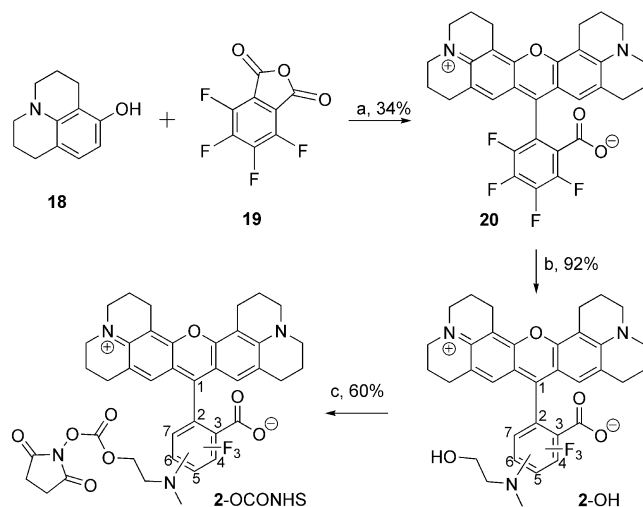
Scheme 6. Tetrafluororhodamine 20 and the amino-reactive NHS carbonate 2-OCONHS : a) C 2 H 3 COOH, TsOH, 160 °C, 16 h; b) CH 3 NH(CH 2 ) 2 OH, DMF, room temp., 12 h; c) bis( N -succinimidyl) carbonate, NEt 3 , DMF, room temp., 3 h.
