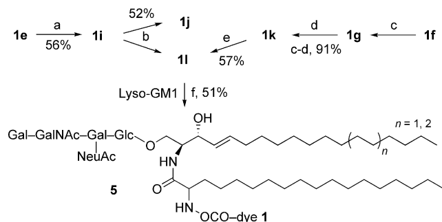
Scheme 3. Synthesis of the labelled \alpha -aminostearic acid 1l and the fluorescent ganglioside GM1 derivative 5 : a) 4 - t BuO, \text{NH}_2 , \text{NEt}_3 , DMF, room temp., 4 d; b) TFA, \text{Et}_3\text{SiH} , \text{CH}_2\text{Cl}_2 , room temp., 24 h; c) bis( N -succinimidyl) carbonate, \text{NEt}_3 , DMAA, room temp., 1 h; d) 4 -MeO, \text{NH}_2 ·HCl, room temp., 48 h; e) LiI, THF, 100 °C, 48 h; f) HATU, \text{NEt}_3 , DMSO, room temp., 24 h.
